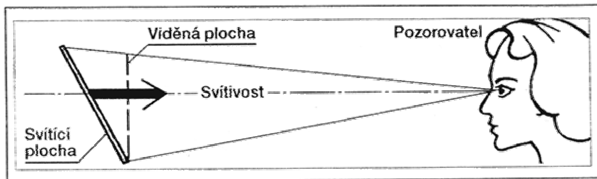
Obr. 2.4 Definice jasu
